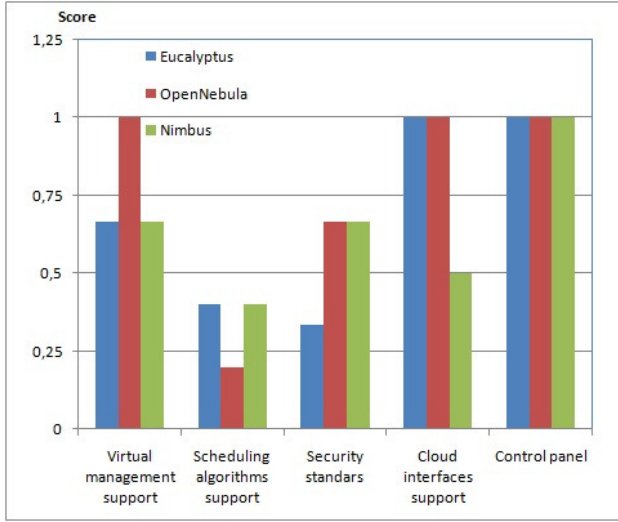
Figure 2. Middleware comparison
